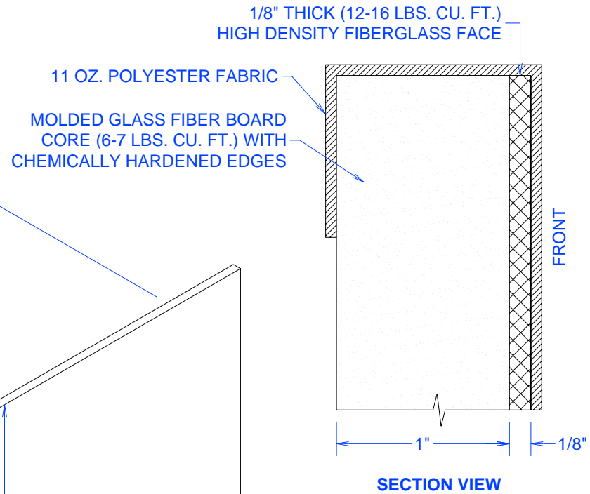
SECTION VIEW
